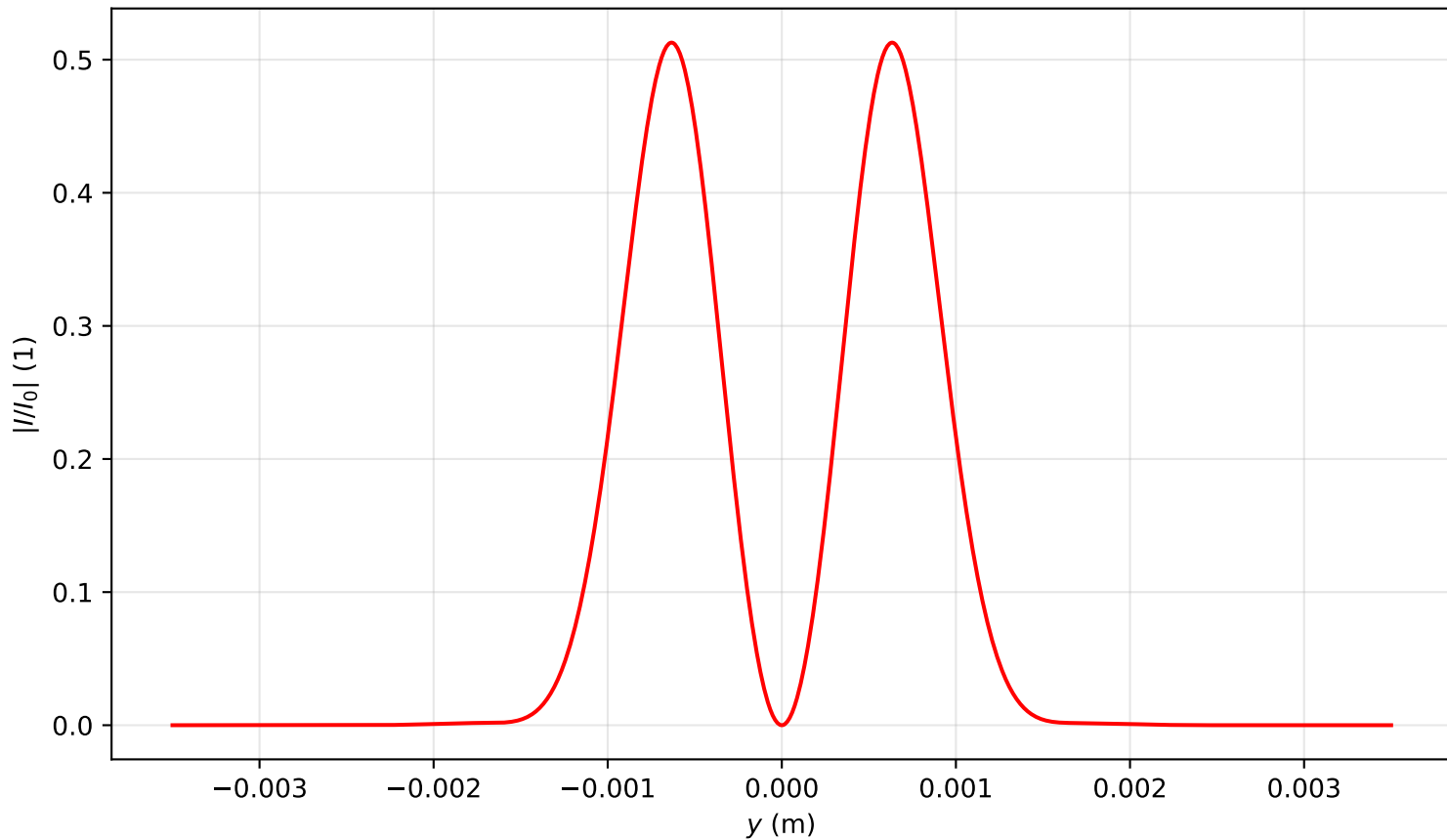
Intensity profile I(x=0, y, z=1.513)/I_0 , P_{in}=2.0P_{cr} , artificial time
